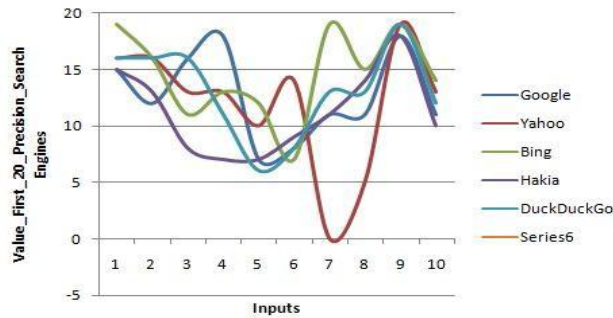
Fig. 4 Visual Representation of Search Engines for first 20 Precision
